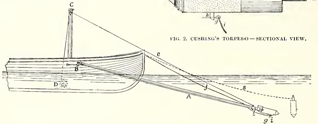
FIG. 1. CUSHING'S LAUNCH AND TORPEDO—SHOWING METHODS OF WORKING.
